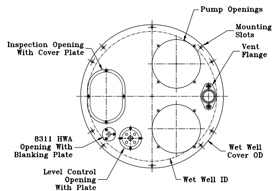
8805 Duplex Round Wet Well Cover Vertical and Submersible Floor Mount Models
